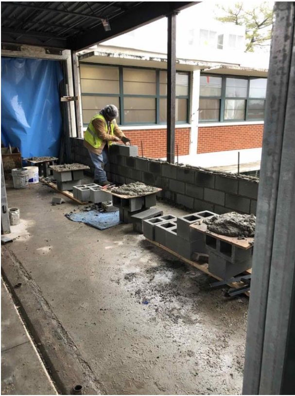
CMU wall at media center
